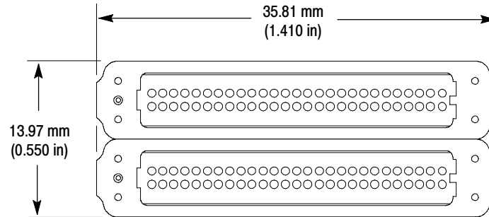
Figure 24: Side-by-side layout
