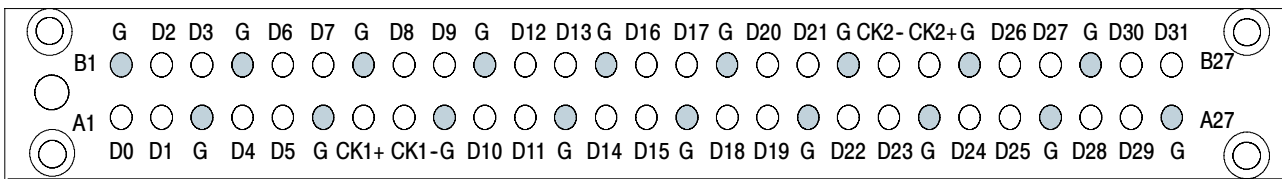
Figure 30: P6960 single-ended PCB footprint pinout detail
