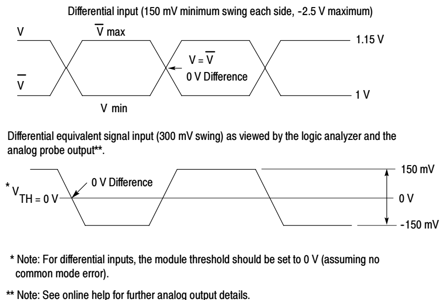
Figure i: Differential input amplitude
