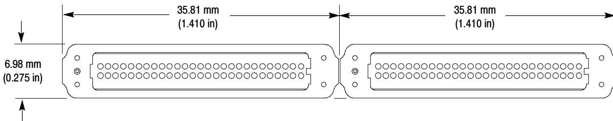
Figure 25: End-to-end layout
