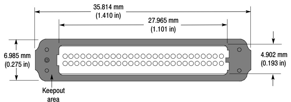
Figure 23: Keepout area
